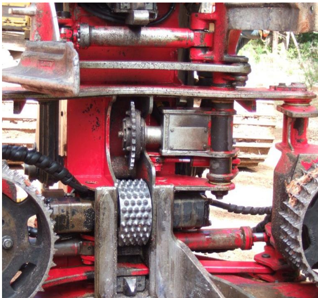
Figure 1. Warratah harvester head with the PH-330 probes highlighted
